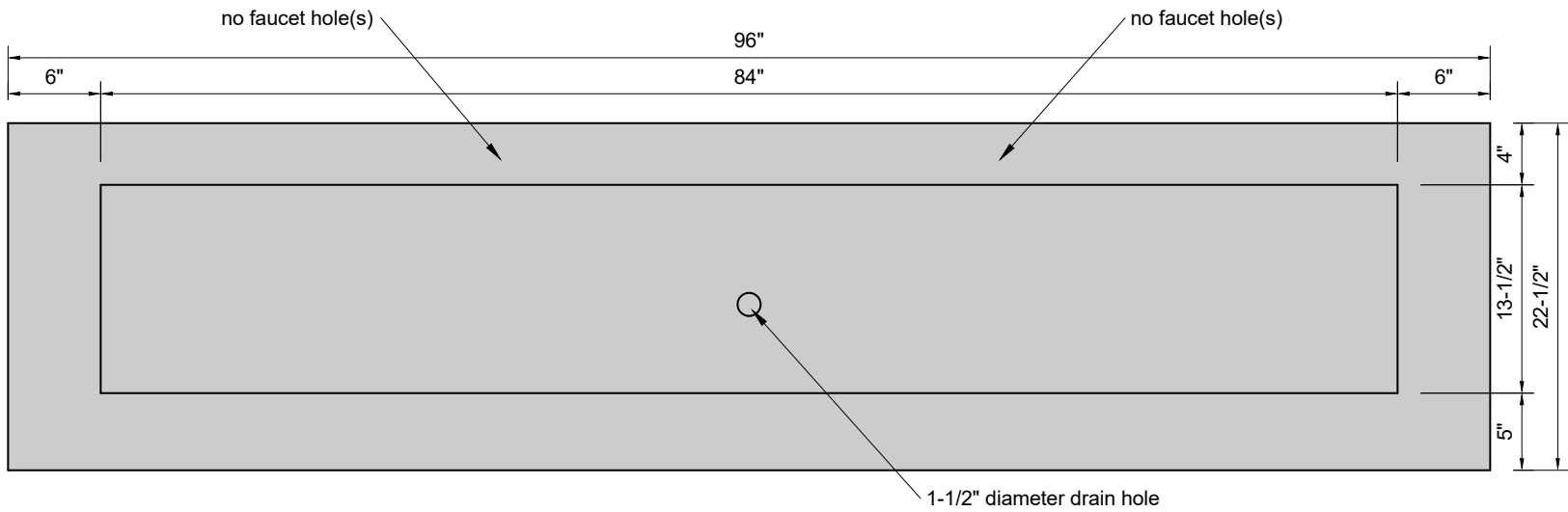
TOP VIEW
