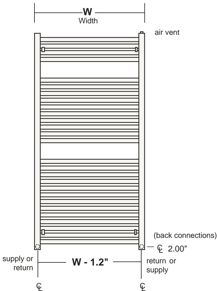
Front View Dimensions
