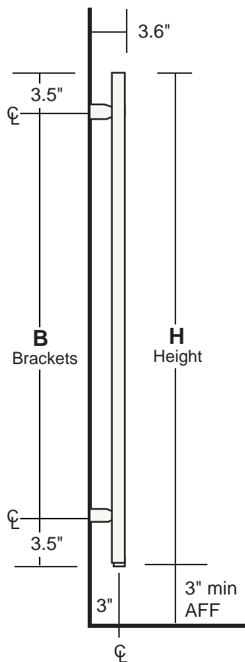
Side View Dimensions
